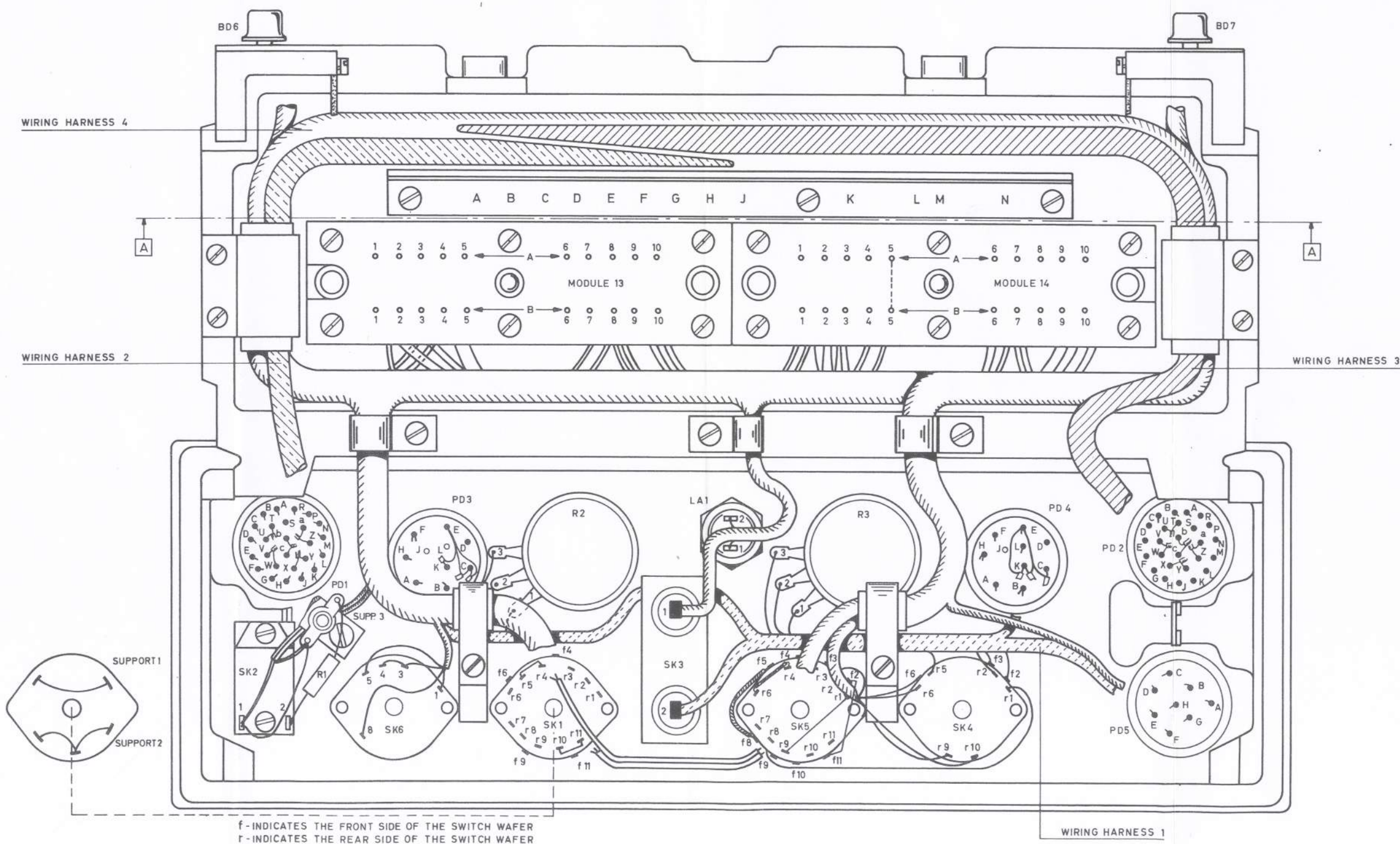
WIRING FRAME ASSEMBLY FIGURE 9
