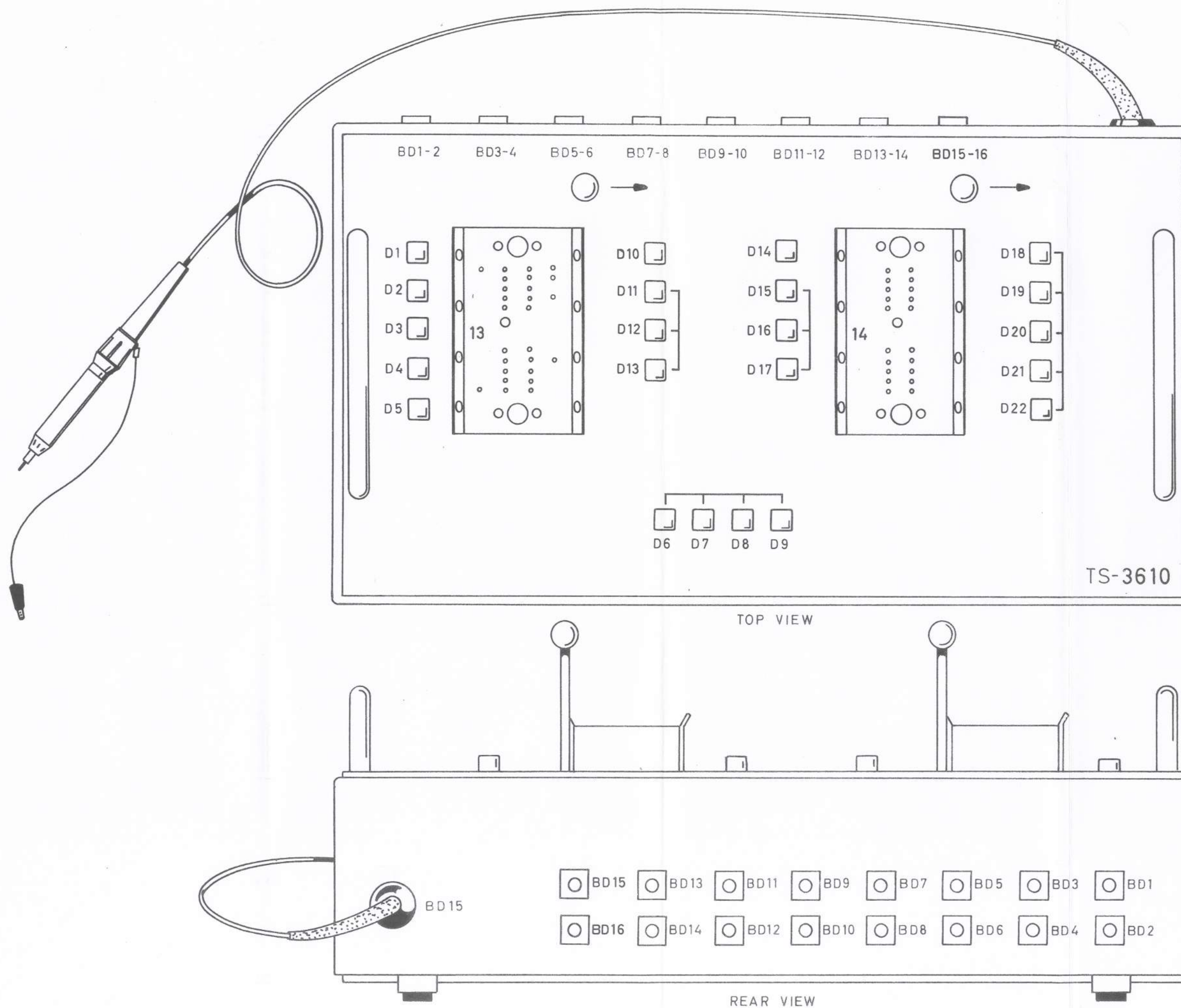
MODULE TESTER TS-3610 FIGURE 6
