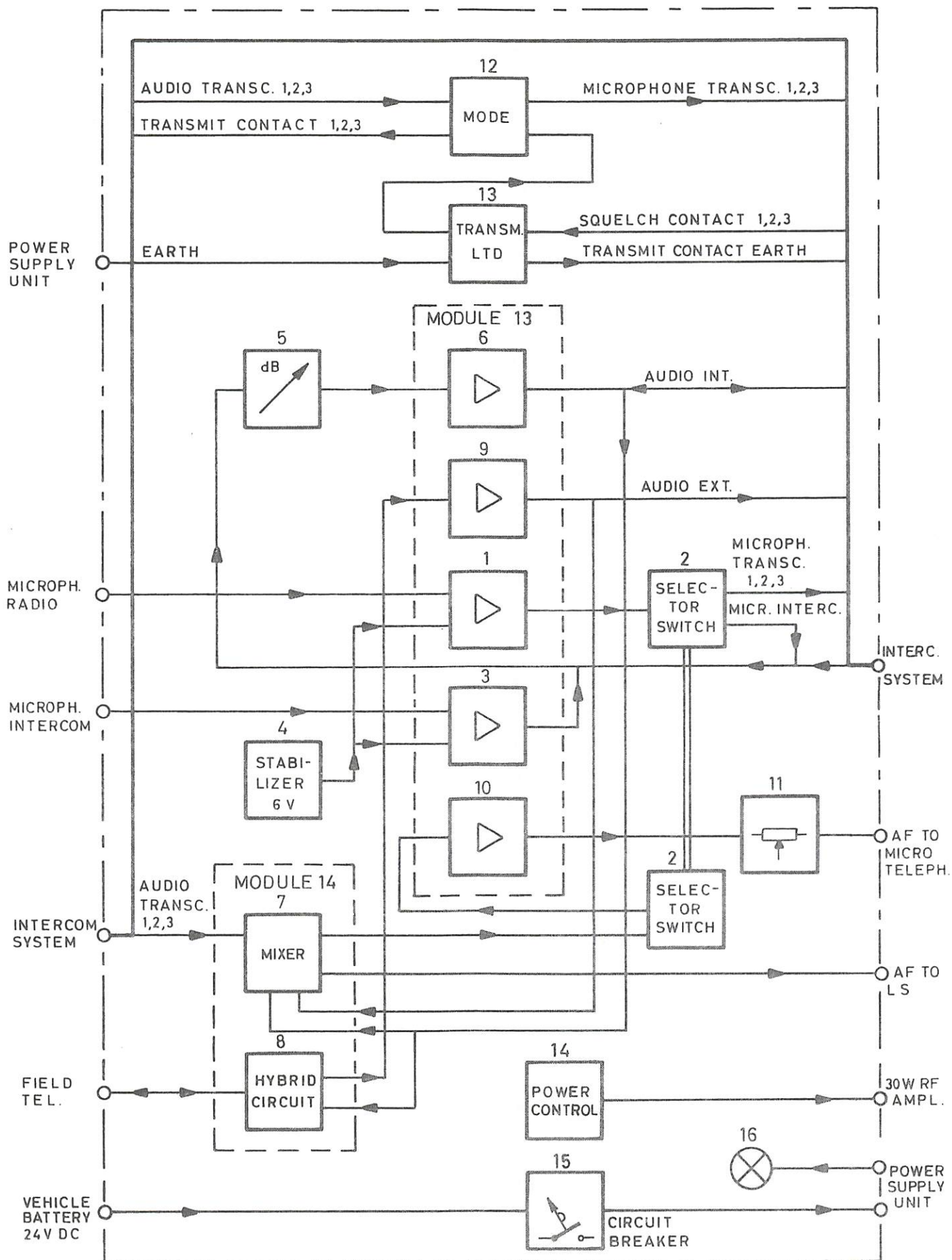
BLOCK DIAGRAM FIGURE 3
