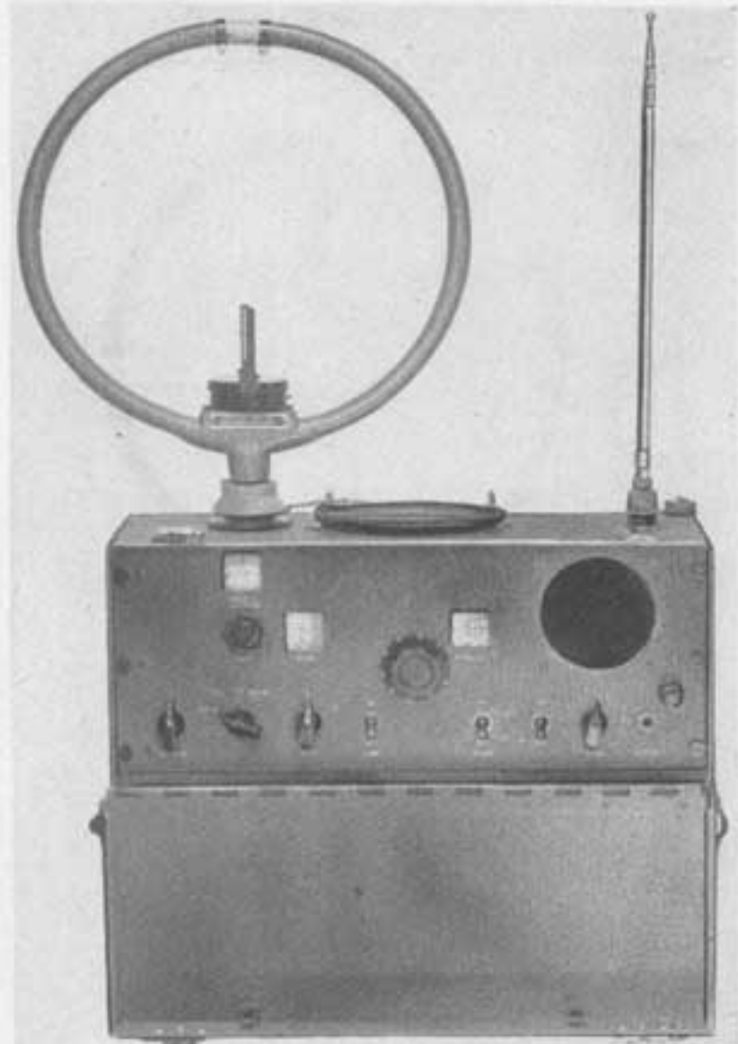
Model DAG-1 portable radio direction-finding equipment.
