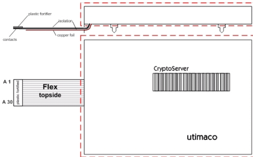
Figure 2 – CryptoServer CSe-Series – side view and top view
