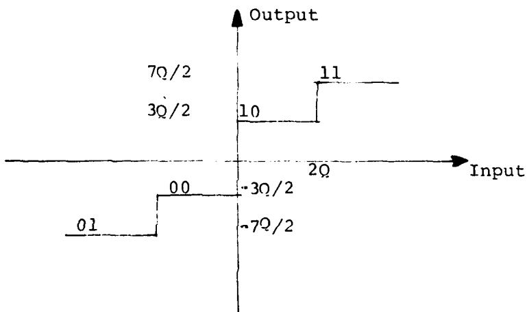
(b) a 2-bit Quantizer
