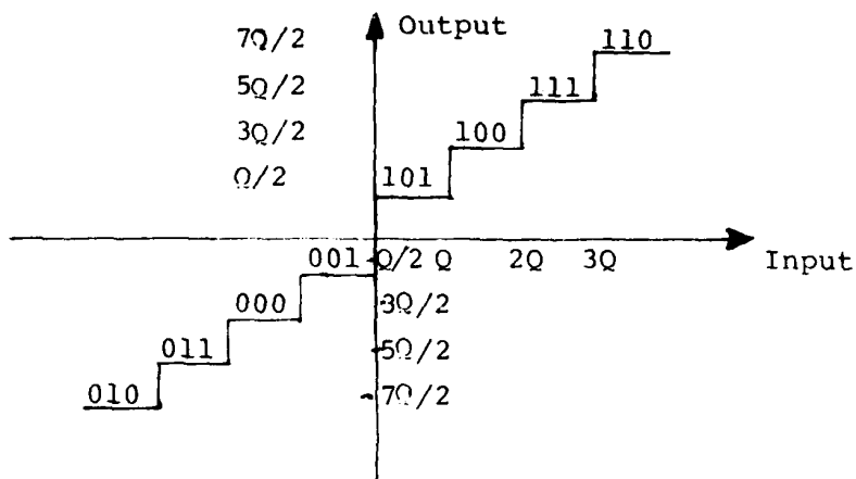
(a) a 3-bit Quantizer
