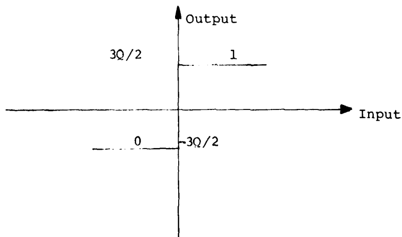
(c) a 1-bit Quantizer
