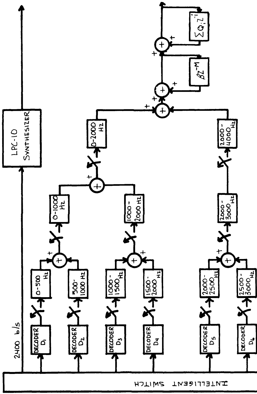
FIGURE 2-10 THE LPC/SBVC MRP RECEIVER
