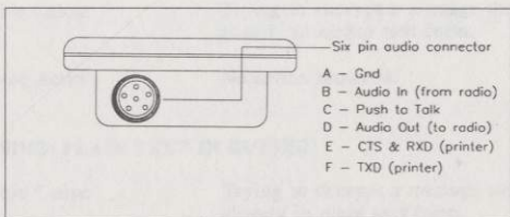
Figure 1: KL-43C Audio Connector
